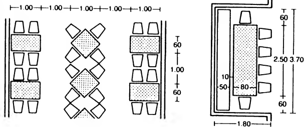
① Minimal seating layout ② Alcoves arrangement
